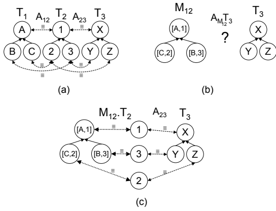
Figure 3: Using the Projection.
