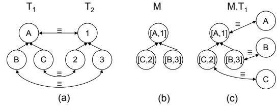
Figure 2: Projecting Taxonomy 1 from the Merge.
