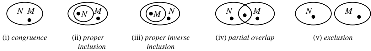
Figure 5: \mathbb{B}_5 – the five basic relations N \equiv M , N \subsetneq M , N \supsetneq M , N \oplus M , N \dot{\perp} M between two sets N, M
